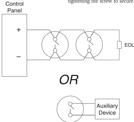
Figure 3. Wiring Diagram – Single Circuit Models
