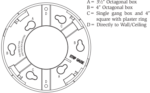
Figure 1. Bracket Mounting Locations
