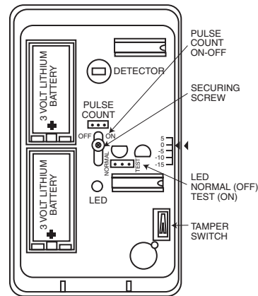
Figure 5. PC Board
