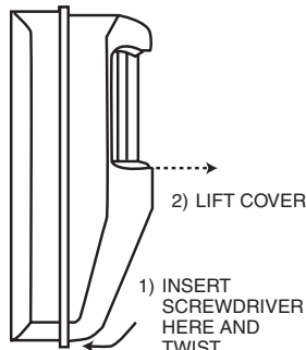
Figure 2. Cover Removal
