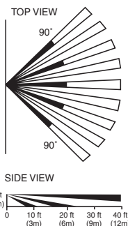
Figure 1. Standard Wide-Angle Protection Pattern
