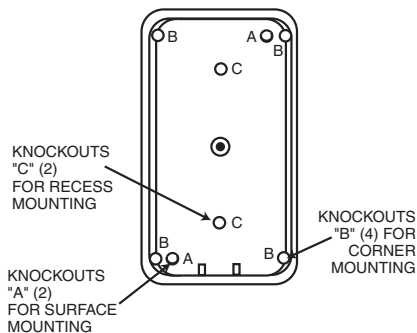
Figure 3. Mounting Holes in Base
