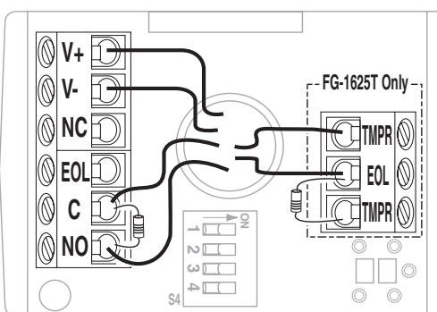
Normally Open Loop/With EOL Resistor
