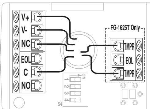
Normally Closed Loop/No EOL Resistor
