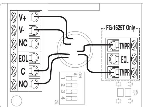
Normally Open Loop/No EOL Resistor
