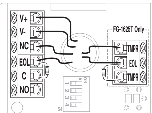
Normally Closed Loop/With EOL Resistor
