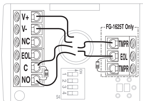
Normally Open Loop/With EOL Resistor
